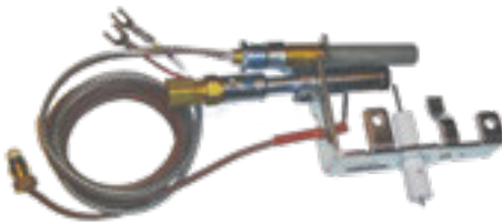
Universal 3/16" Male (Thermocouple is Metric Thread)
